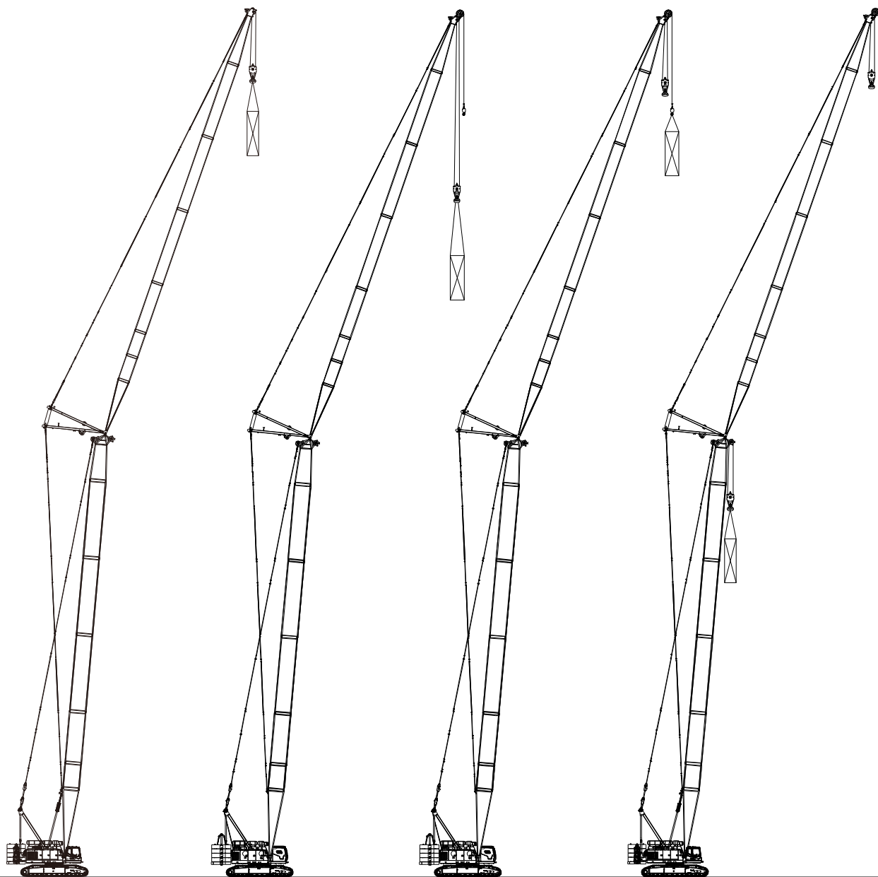
LJ Configuration (single hook, load on luffing jib hook) LJm Configuration (double hooks, load on luffing jib hook) LJa Configuration (double hooks, load on extension jib hook) LJCZG Configuration (double hooks, load on main hook)
