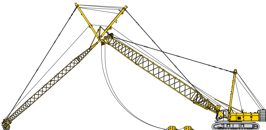
Erecting of main boom and luffing jib
